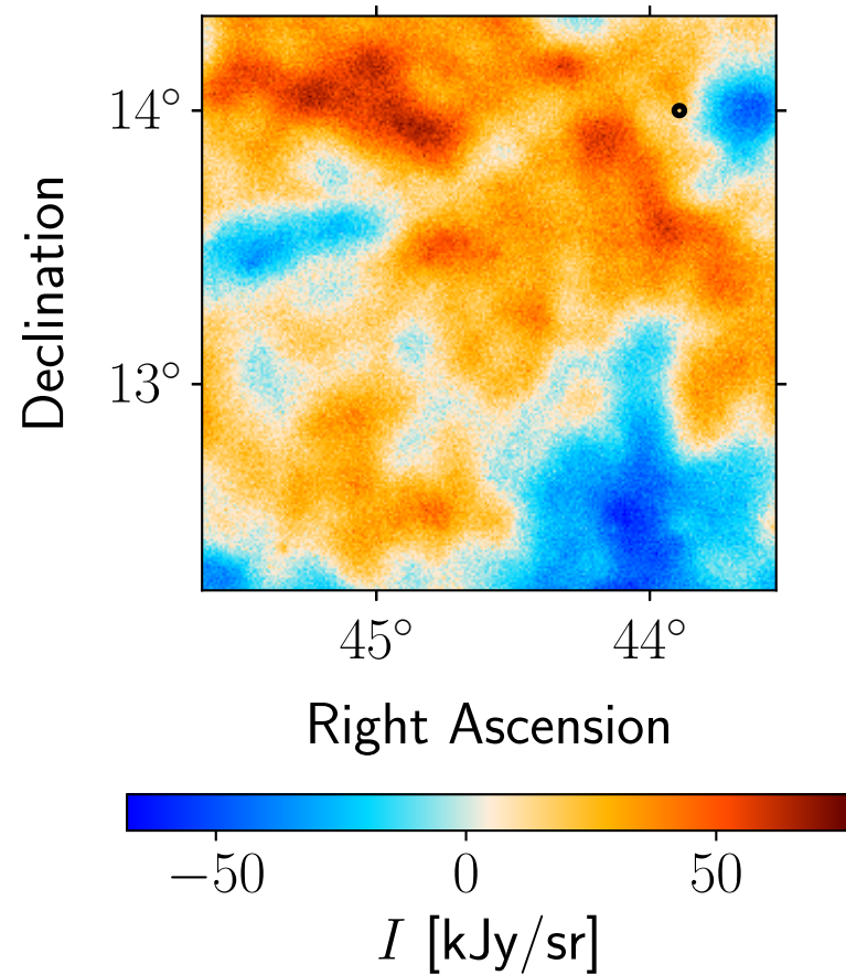
Residual: ACT 98 GHz
