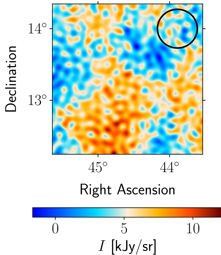
Residual: Planck 30 GHz
