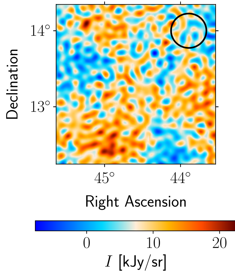
Residual: Planck 44 GHz
