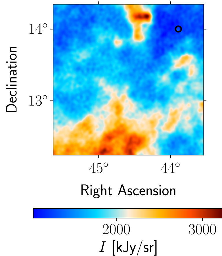
Residual: Planck 545 GHz
