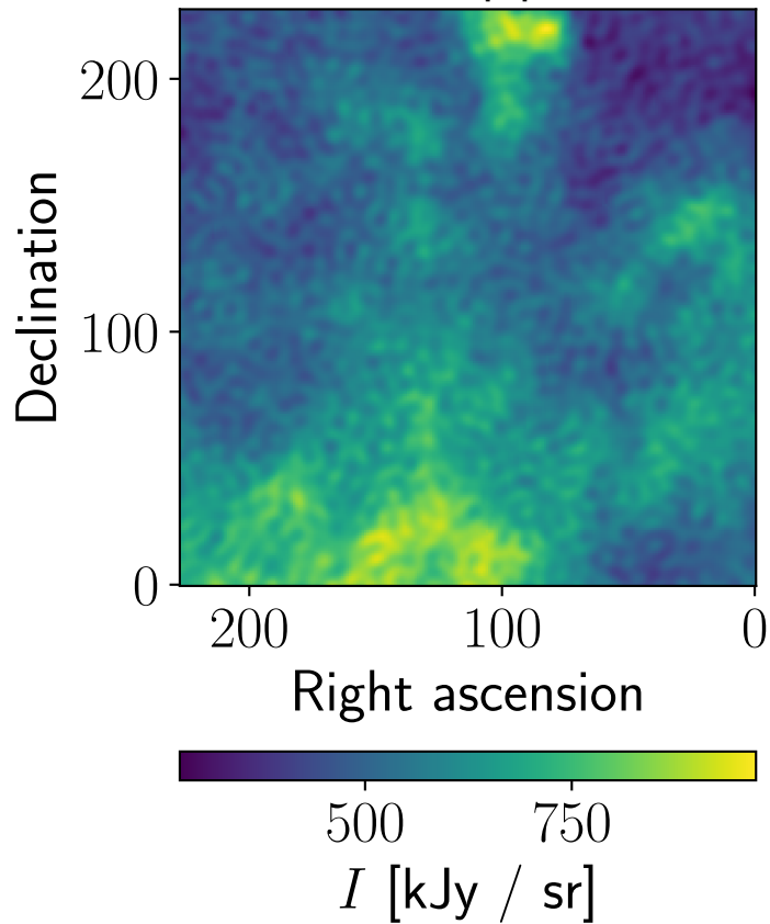
Data, Planck, npipe, 353 GHz
