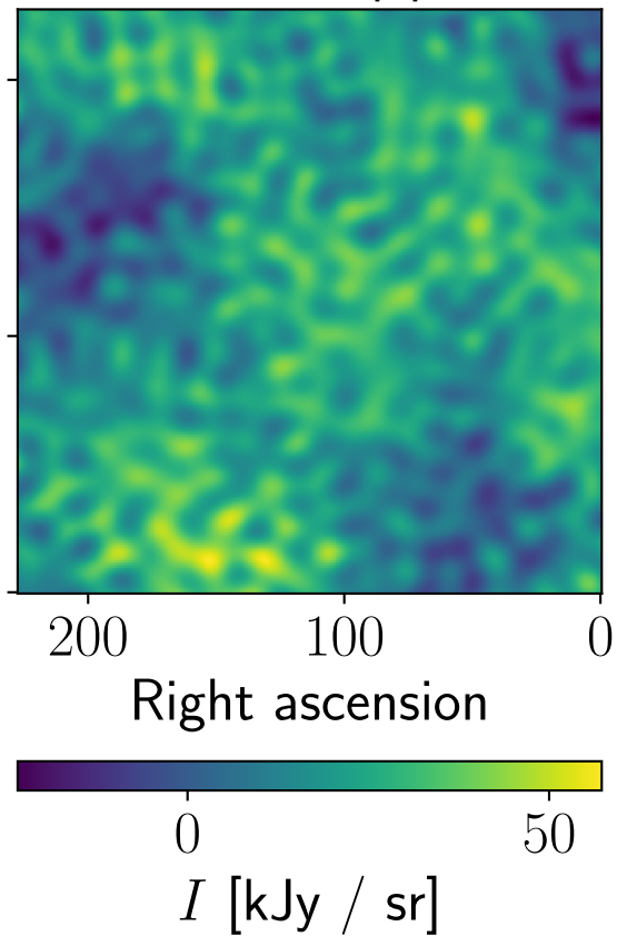
Residual, Planck, npipe, 70 GHz
