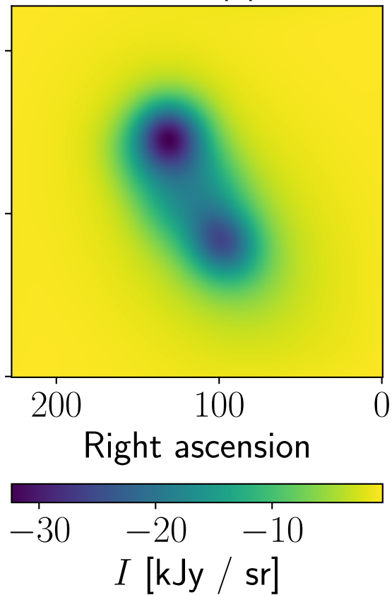
Model, Planck, npipe, 70 GHz
