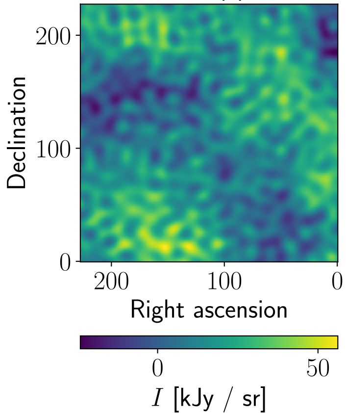
Data, Planck, npipe, 70 GHz
