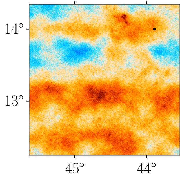
Data: ACT 220 GHz
