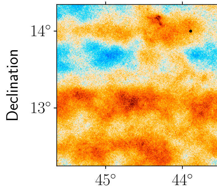
Residual: ACT 220 GHz
