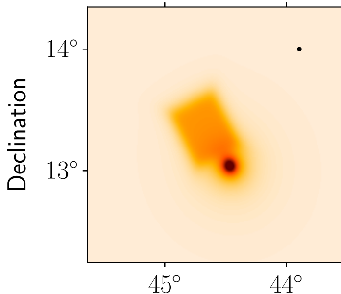
Model: ACT 220 GHz
