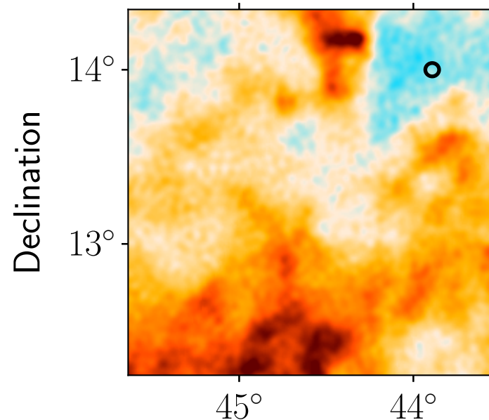
Residual: Planck 545 GHz
