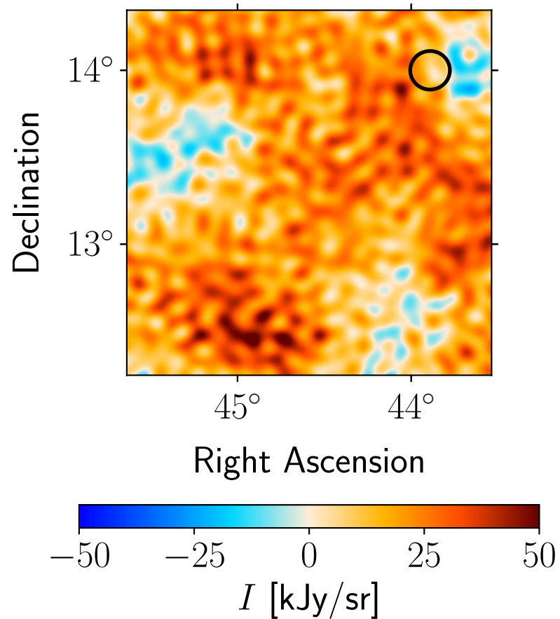
Residual: Planck 70 GHz
