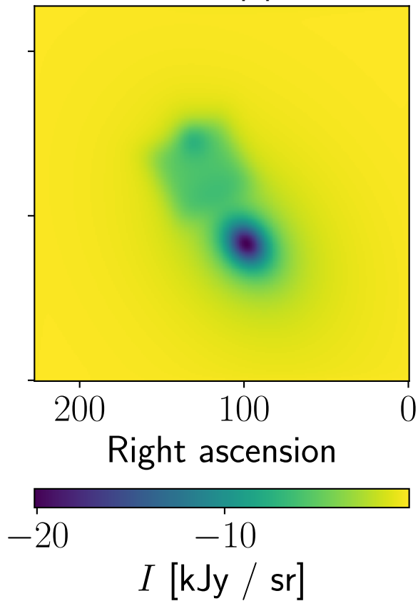
Model, Planck, npipe, 217 GHz
