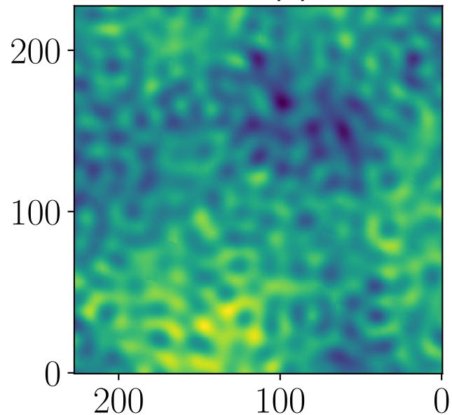
Data, Planck, npipe, 30 GHz
