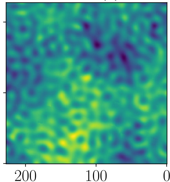
Residual, Planck, npipe, 30 GHz
