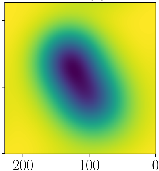
Model, Planck, npipe, 30 GHz
