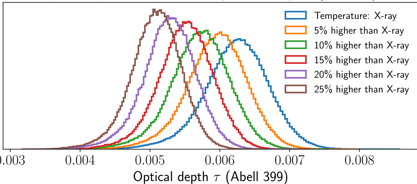
Optical depth vs temperature for system velocity fits (Abell 399)
