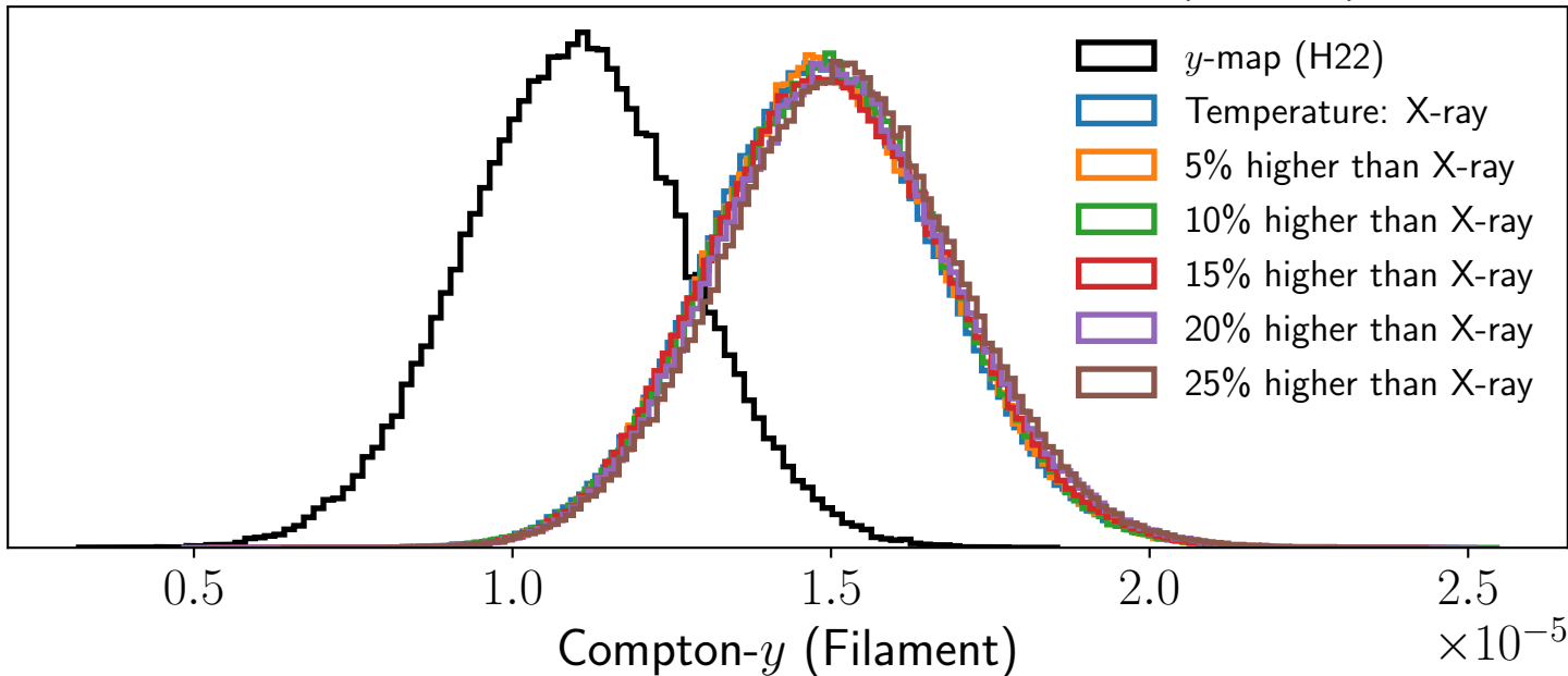
Compton- y vs temperature for system velocity fits (filament)
