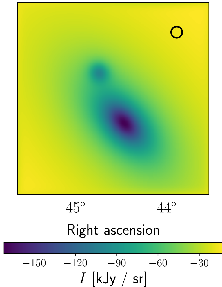
Model, Planck , 143 GHz
