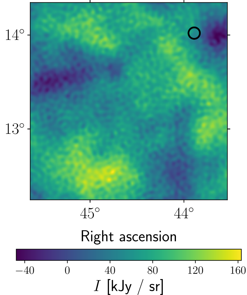
Data, Planck , 143 GHz
