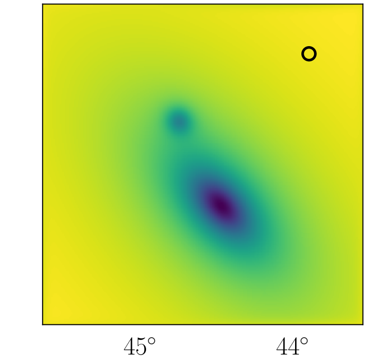
Model, Planck , 217 GHz
