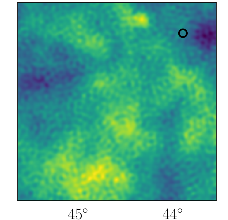
Residual, Planck , 217 GHz
