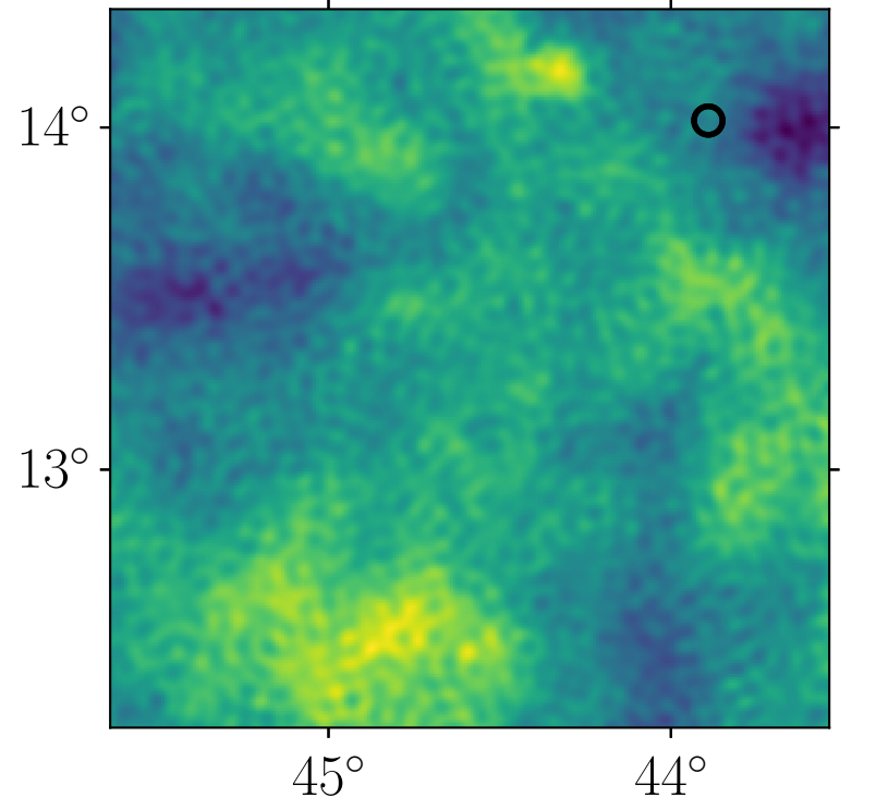
Data, Planck , 217 GHz
