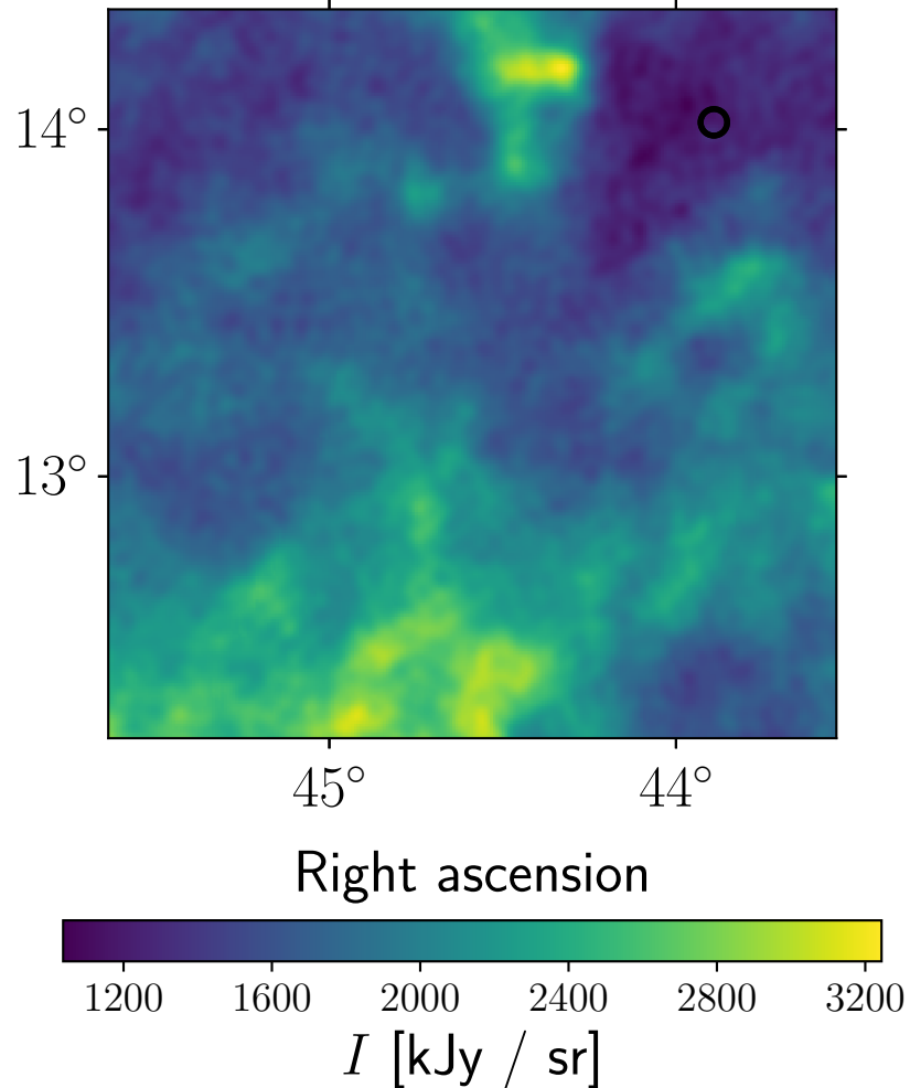
Data, Planck , 545 GHz
