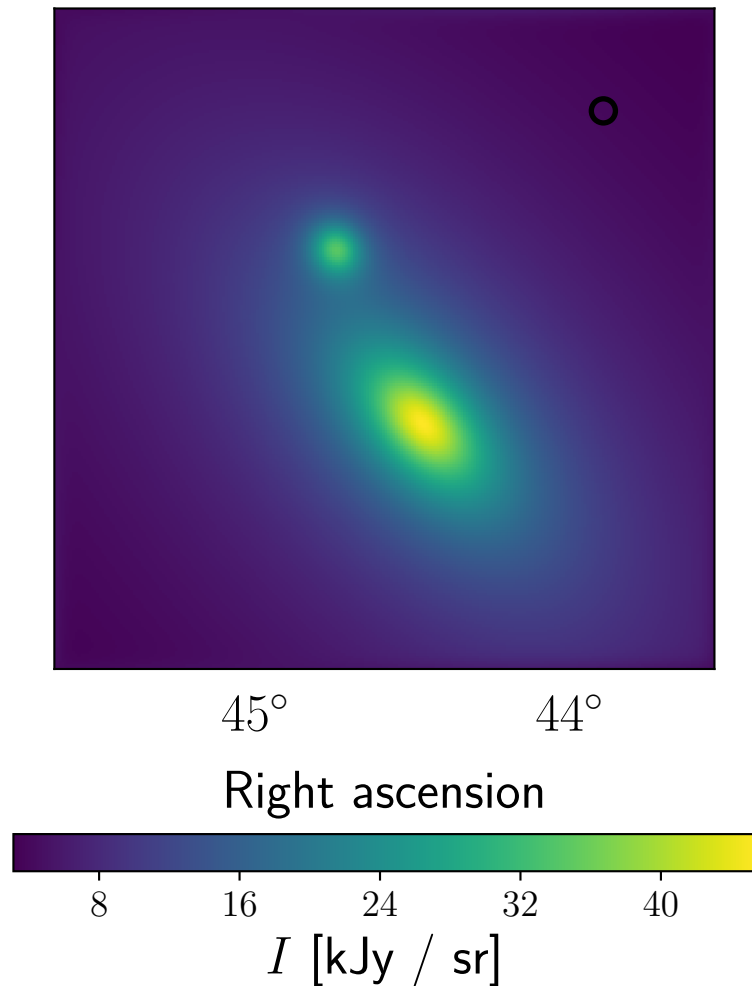
Model, Planck , 545 GHz
