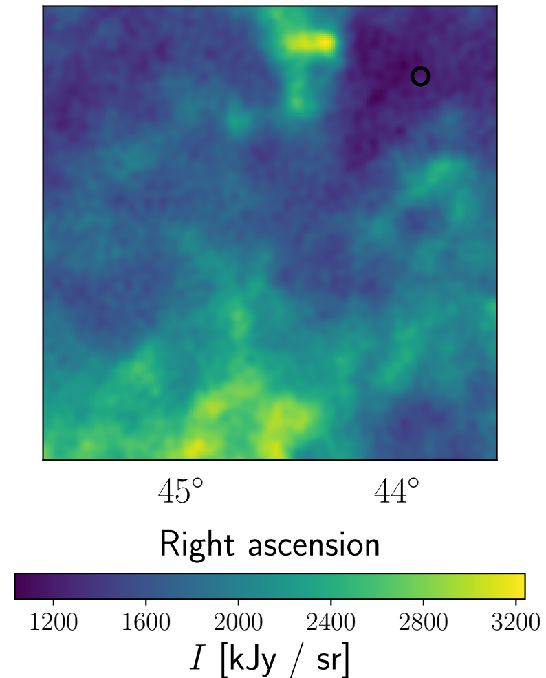
Residual, Planck , 545 GHz
