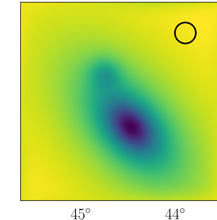
Model, Planck , 70 GHz
