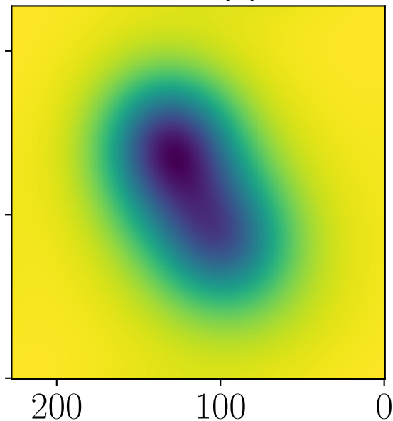
Model, Planck, npipe, 44 GHz
