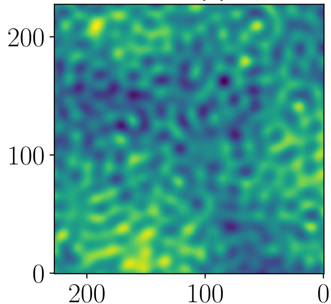
Data, Planck, npipe, 44 GHz
