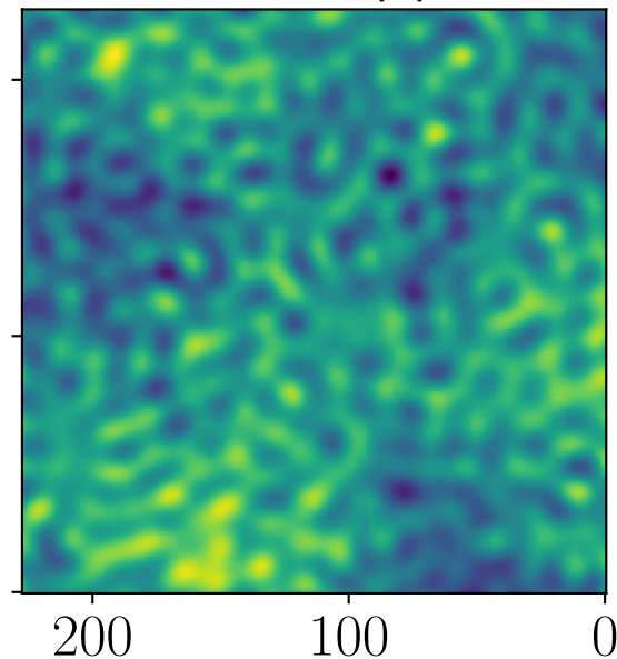
Residual, Planck, npipe, 44 GHz
