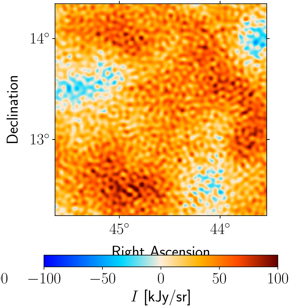
Residual: Planck 100 GHz
