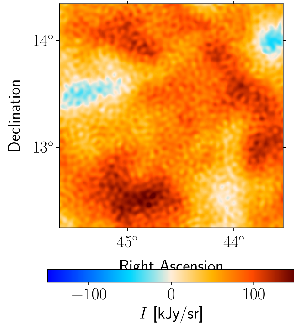
Residual: Planck 143 GHz
