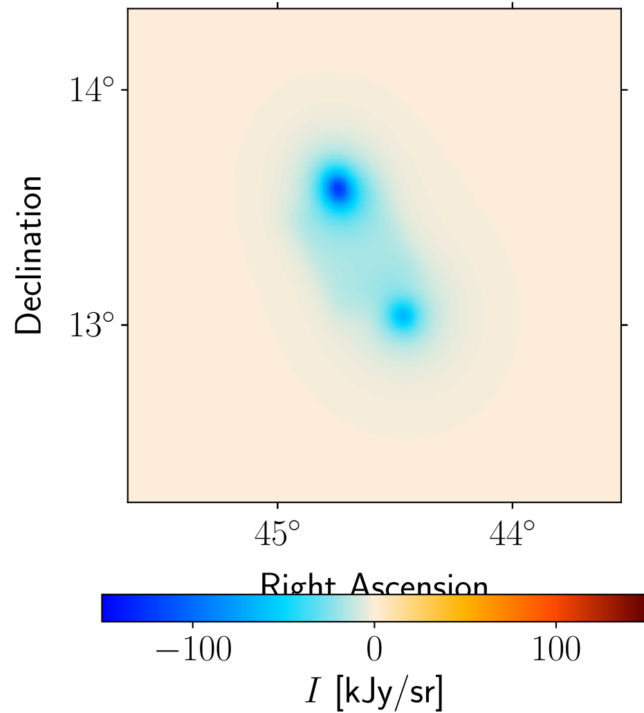
Model: ACT 150 GHz
