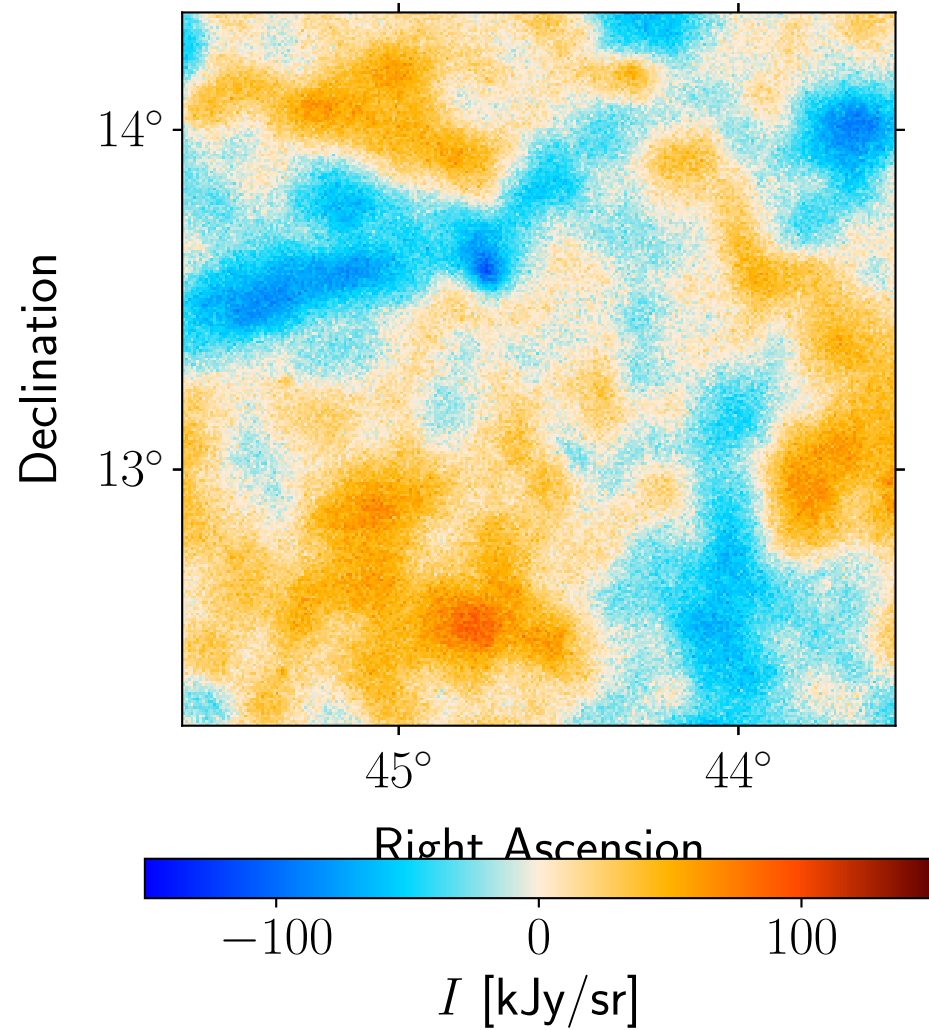
Data: ACT 150 GHz
