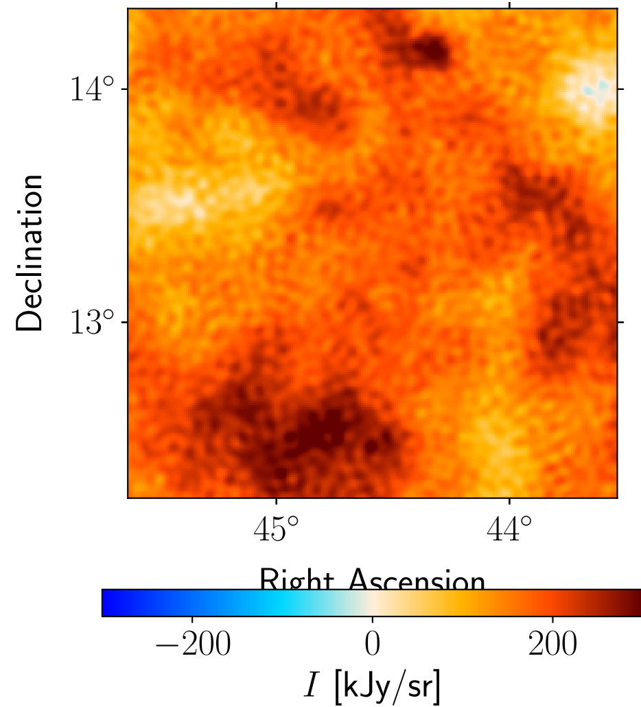
Residual: Planck 217 GHz
