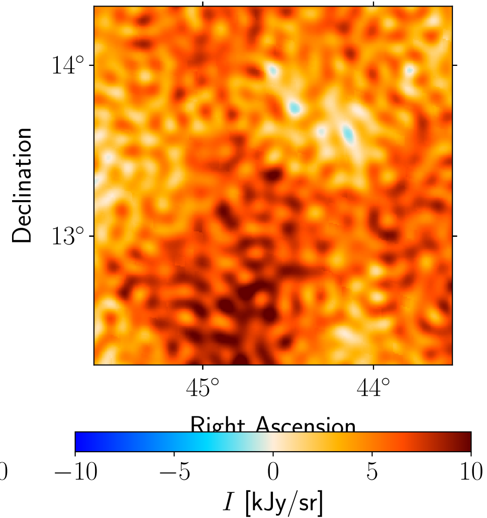
Residual: Planck 30 GHz
