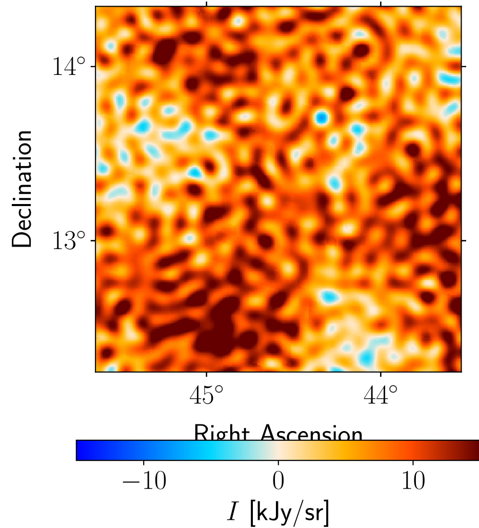
Residual: Planck 44 GHz
