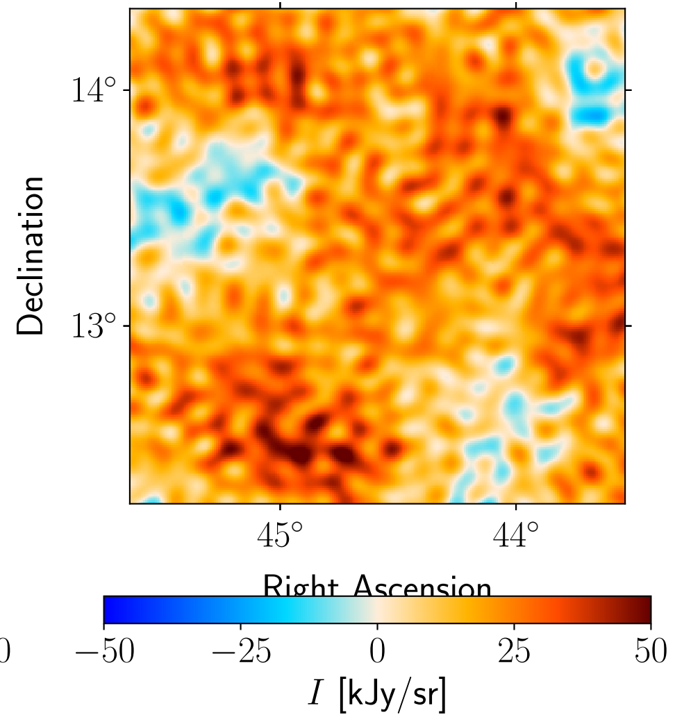
Residual: Planck 70 GHz
