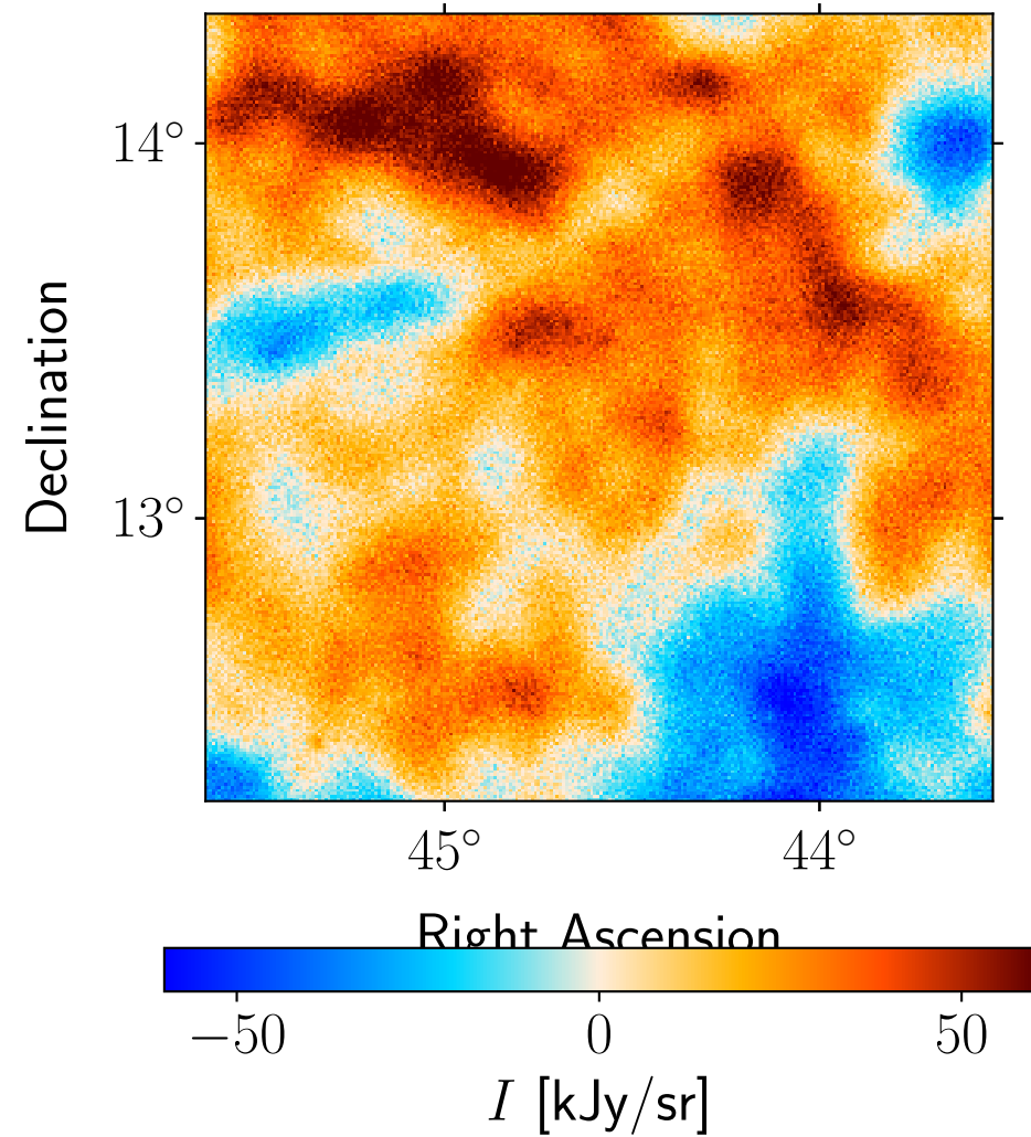
Residual: ACT 98 GHz
