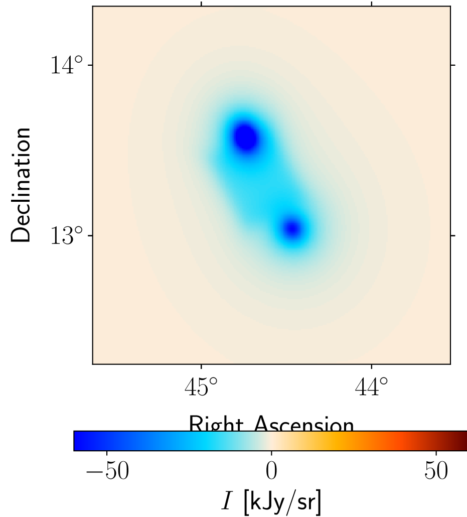
Model: ACT 98 GHz
