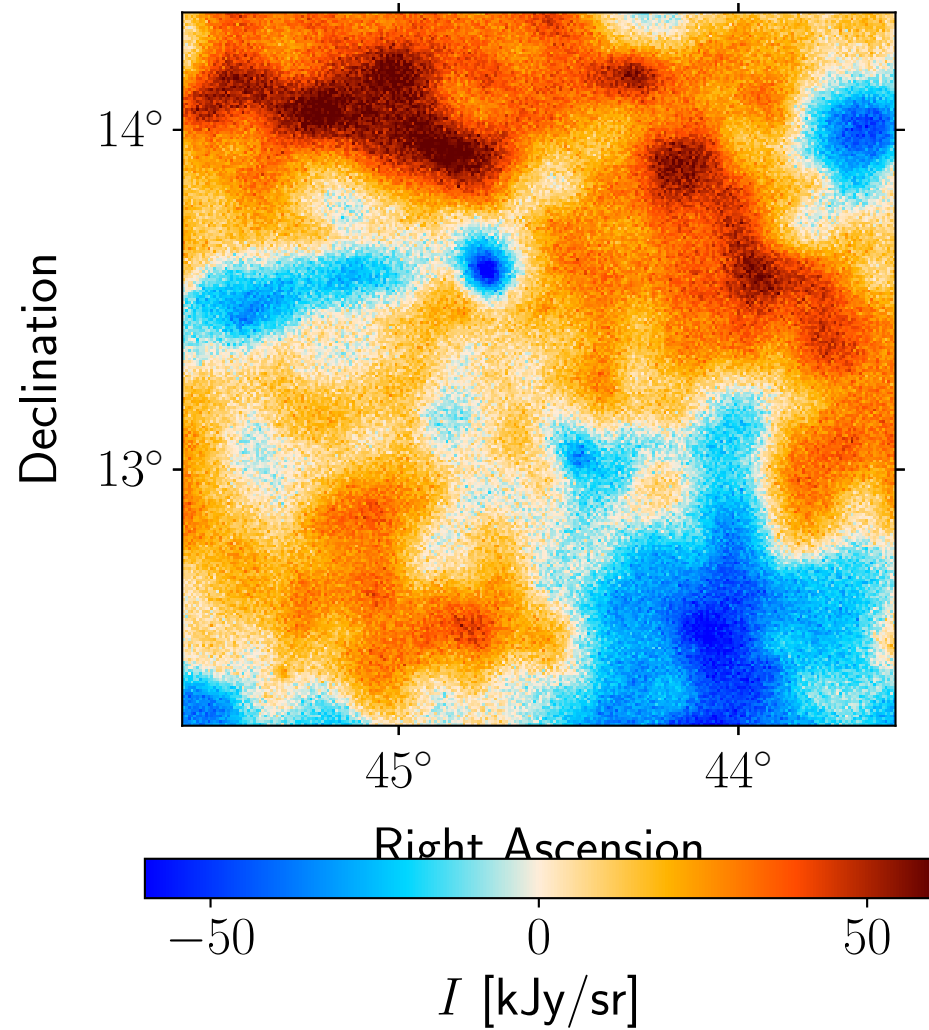
Data: ACT 98 GHz
