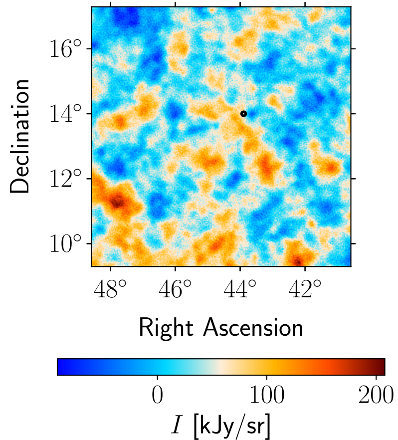
Residual: Planck 143 GHz
