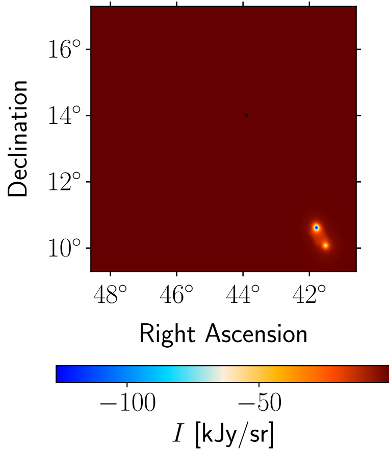
Model: ACT 150 GHz
