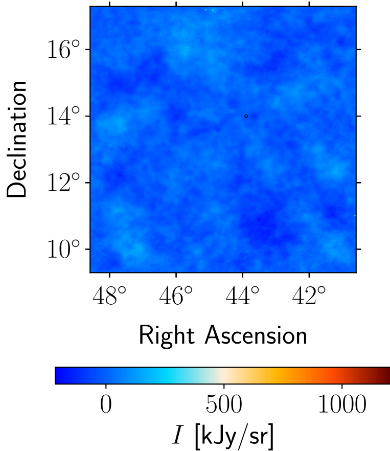
Data: ACT 150 GHz
