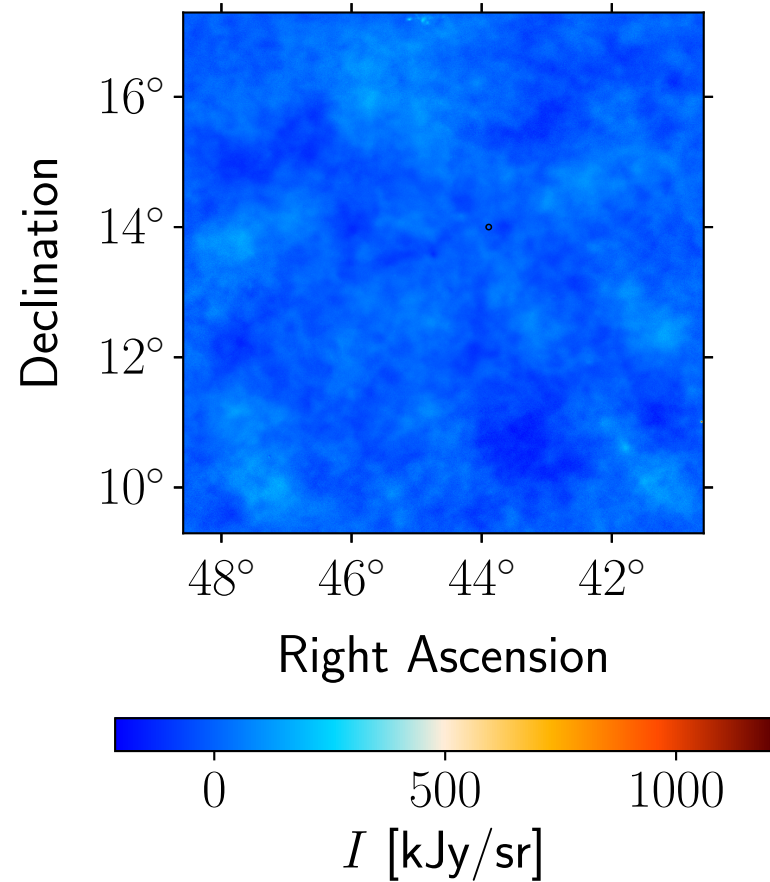
Residual: ACT 150 GHz
