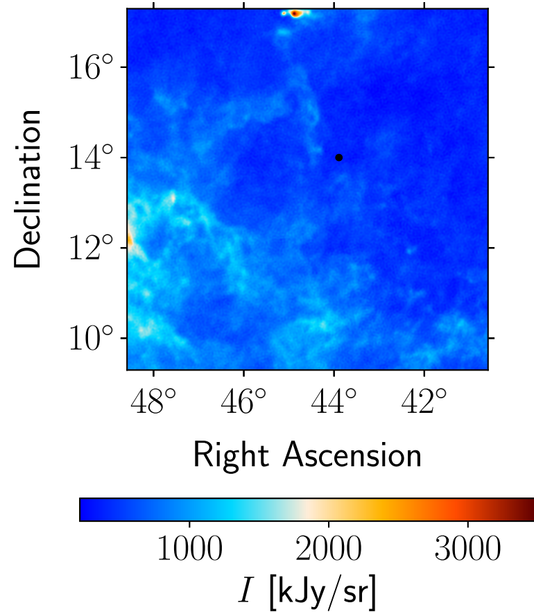
Residual: Planck 353 GHz
