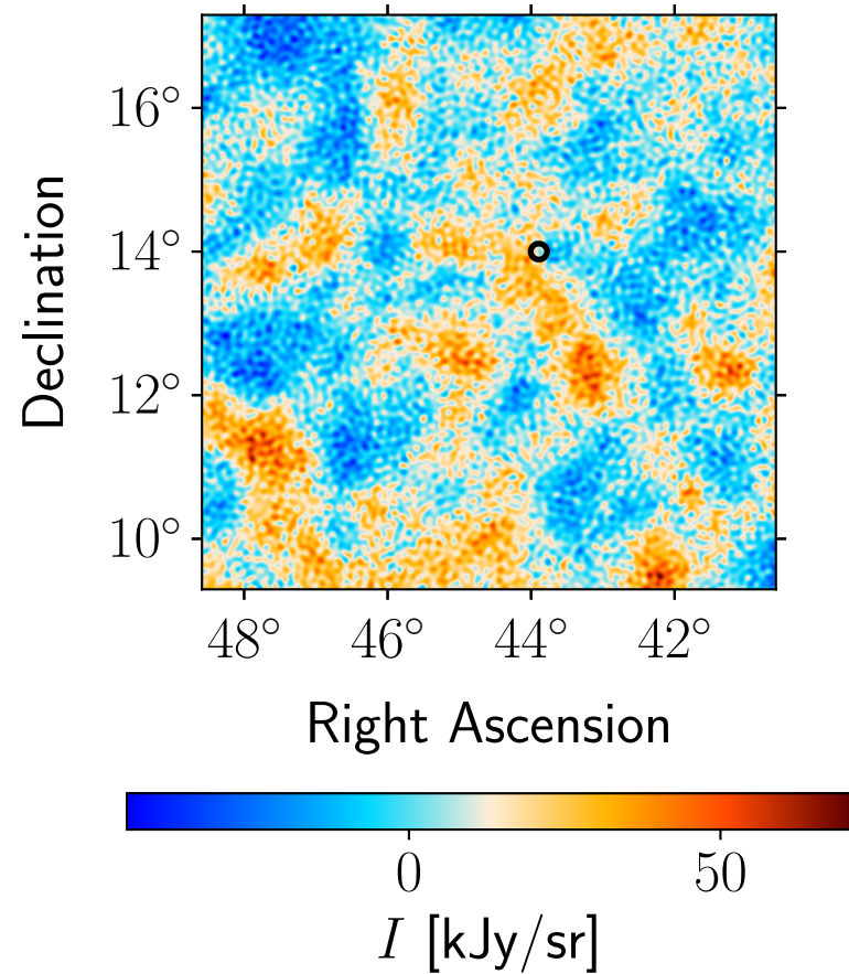
Residual: Planck 70 GHz
