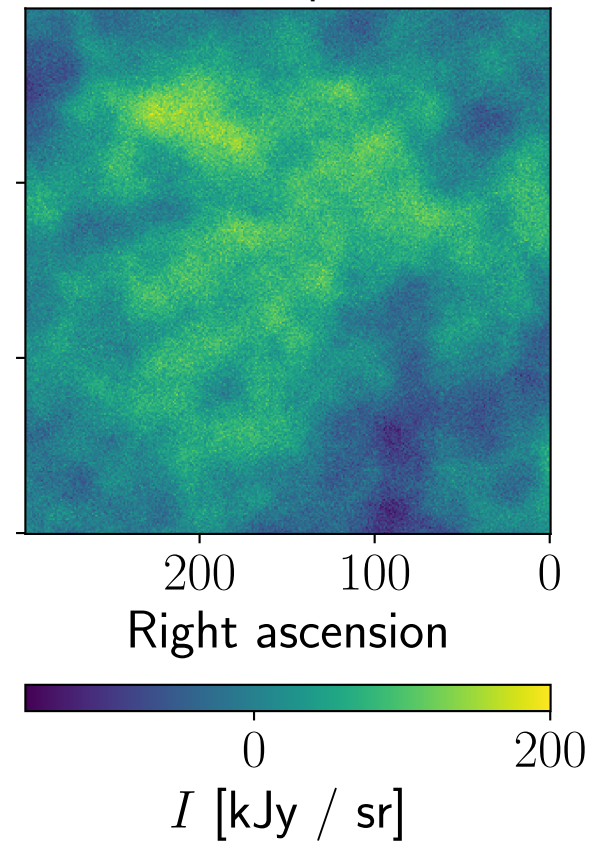
Residual, ACT, pa5, 150 GHz
