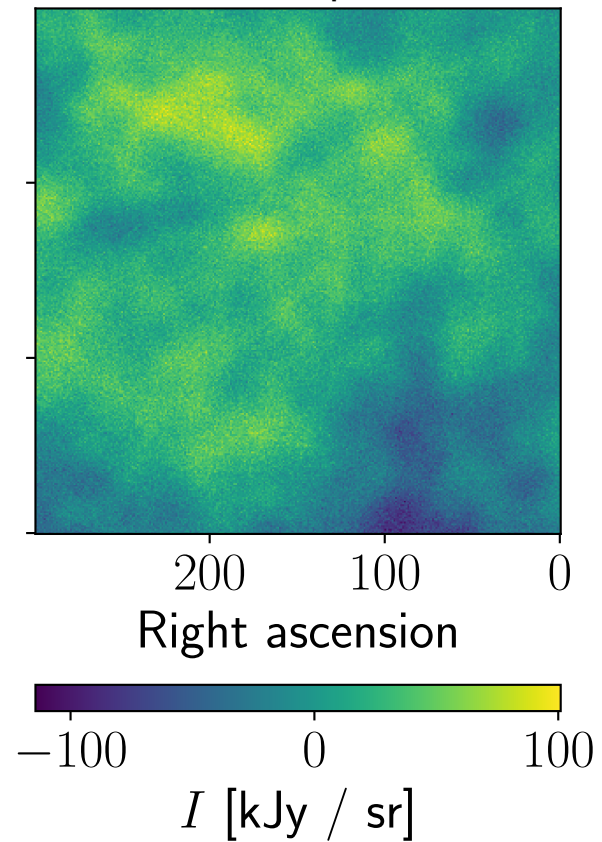
Residual, ACT, pa5, 98 GHz
