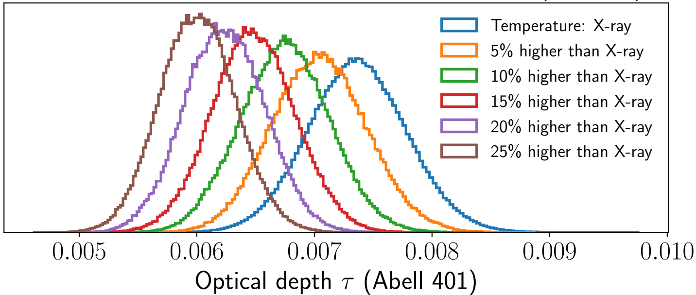
Optical depth vs temperature for individual velocity fits (Abell 401)
