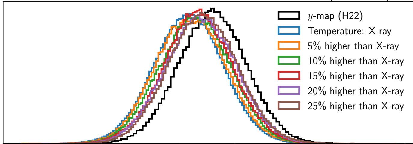
Compton- y vs temperature for individual velocity fits (Abell 401)
