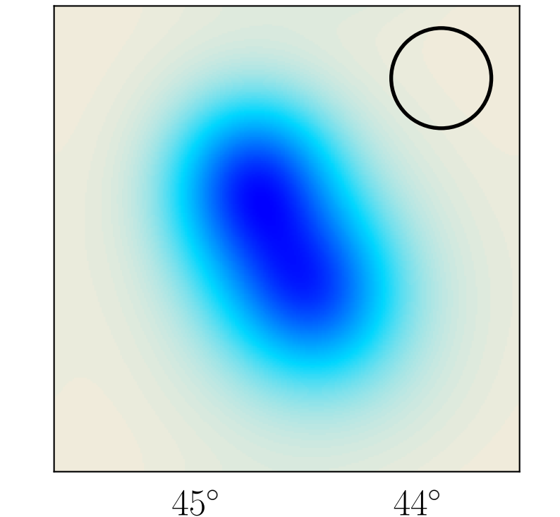
Model, Planck , 44 GHz
