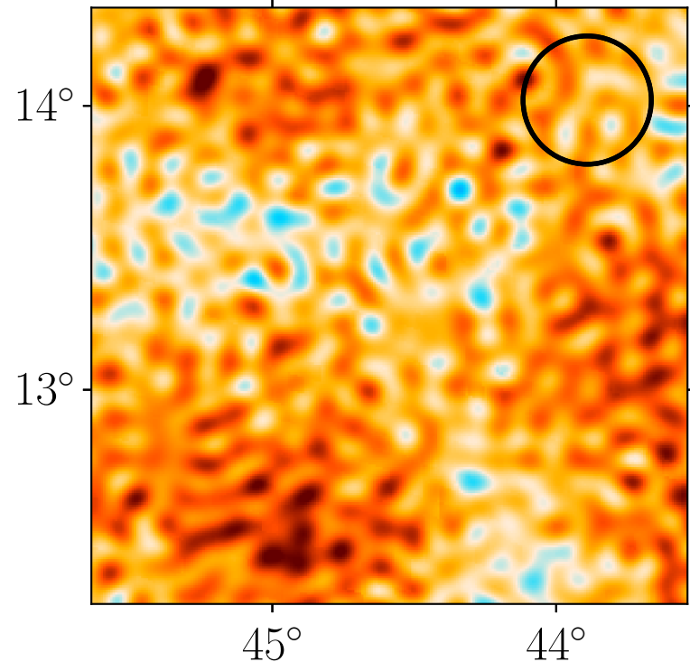
Data, Planck , 44 GHz
