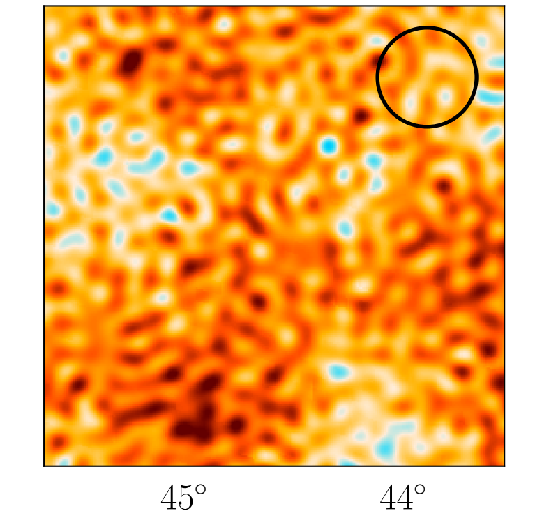
Residual, Planck , 44 GHz
