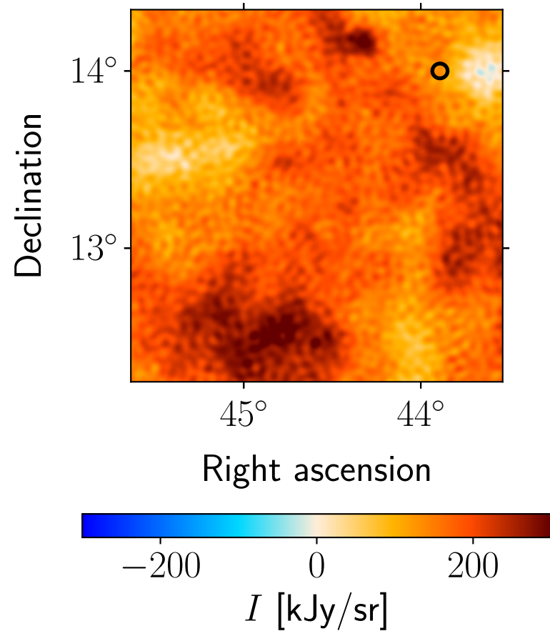
Residual: Planck 217 GHz
