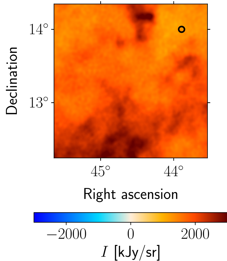
Residual: Planck 545 GHz
