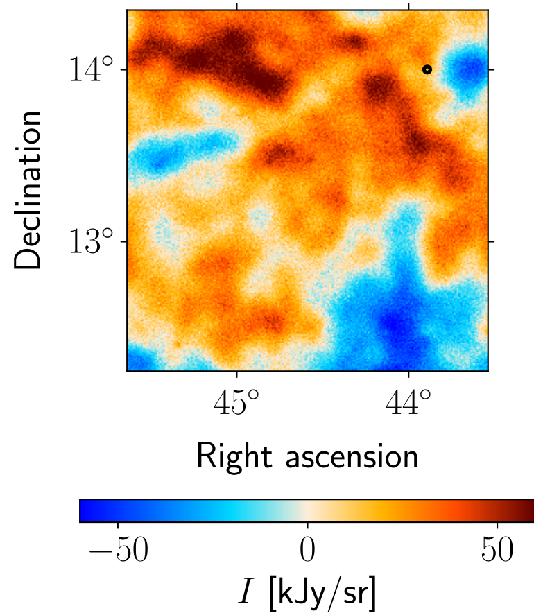
Residual: ACT 98 GHz
