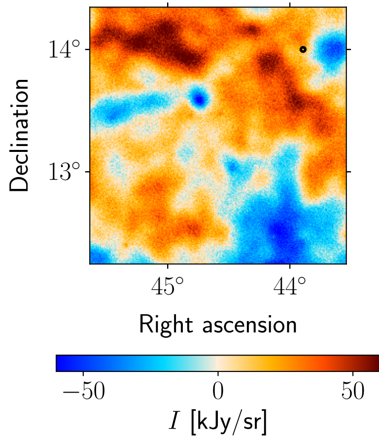
Data: ACT 98 GHz
