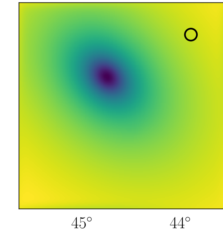
Model, Planck , 143 GHz
