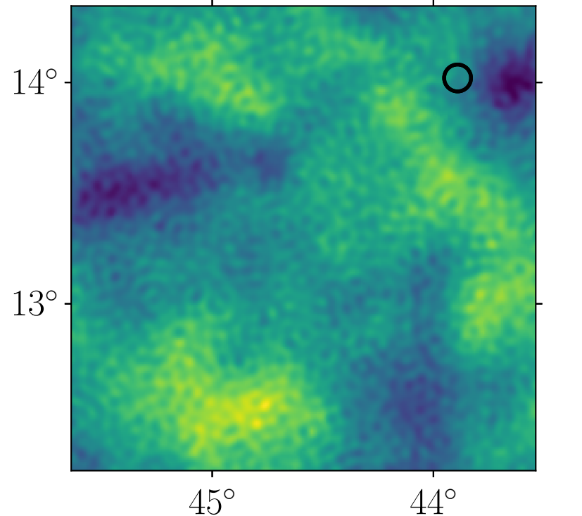
Data, Planck , 143 GHz
