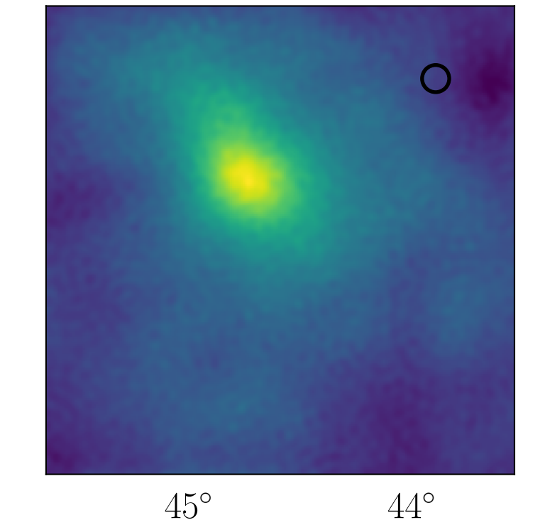
Residual, Planck , 143 GHz
