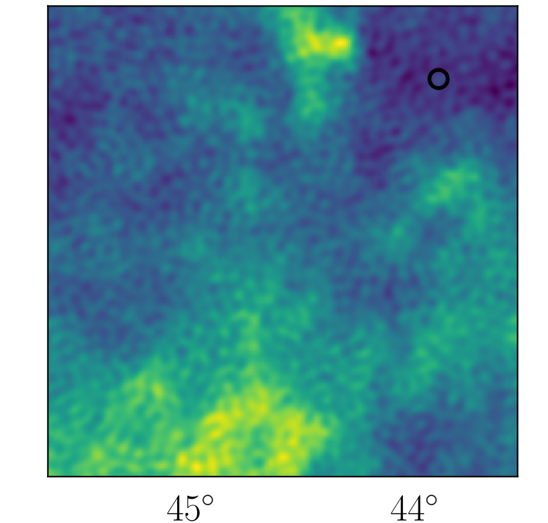
Residual, Planck , 353 GHz
