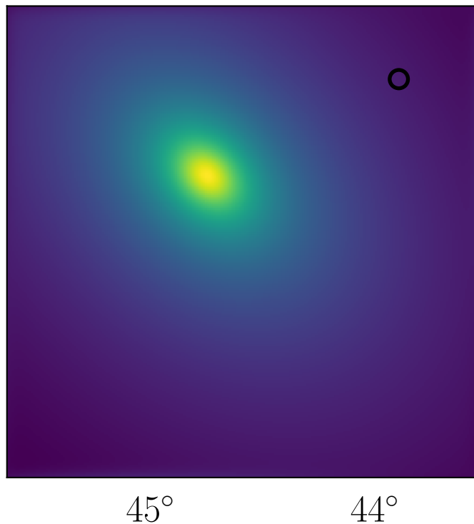
Model, Planck , 353 GHz
