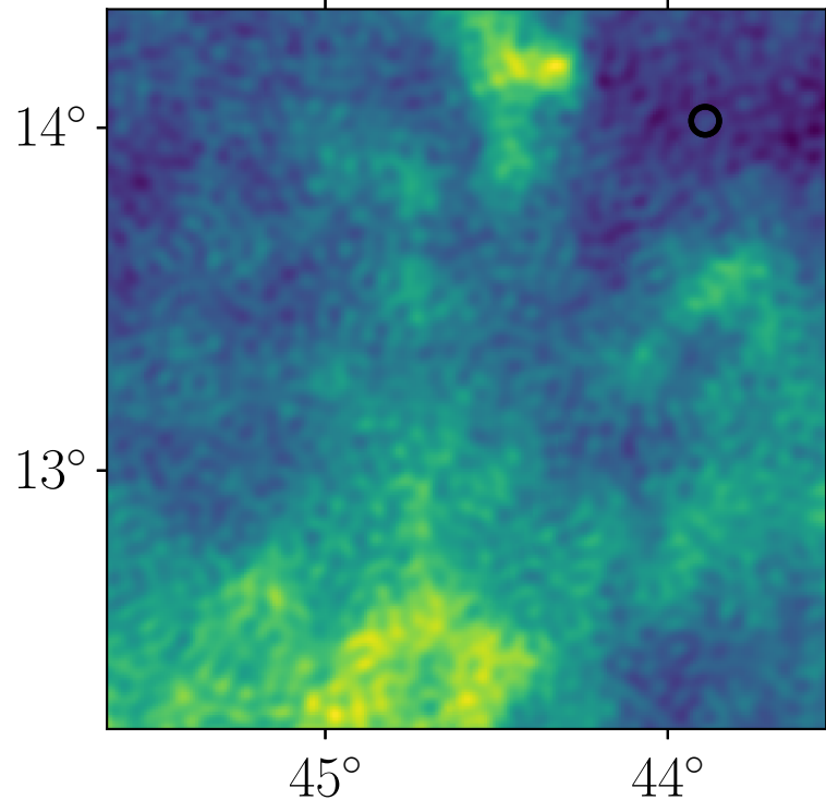
Data, Planck , 353 GHz
