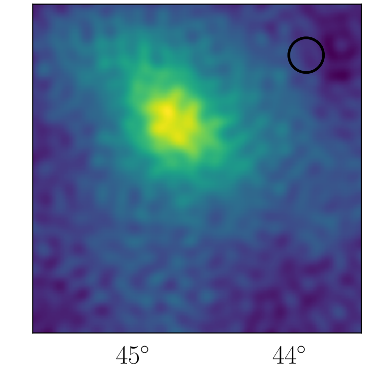
Residual, Planck , 70 GHz
