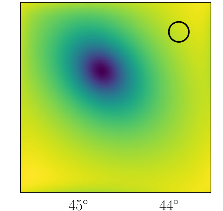
Model, Planck , 70 GHz
