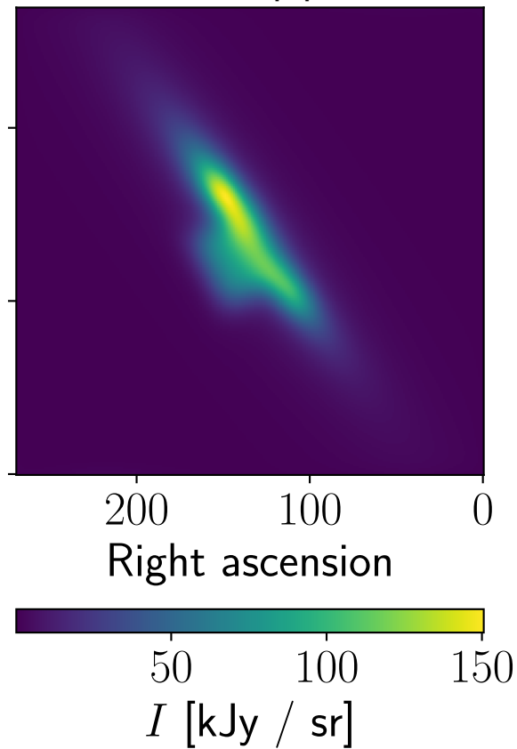
Model, Planck, npipe, 143 GHz
