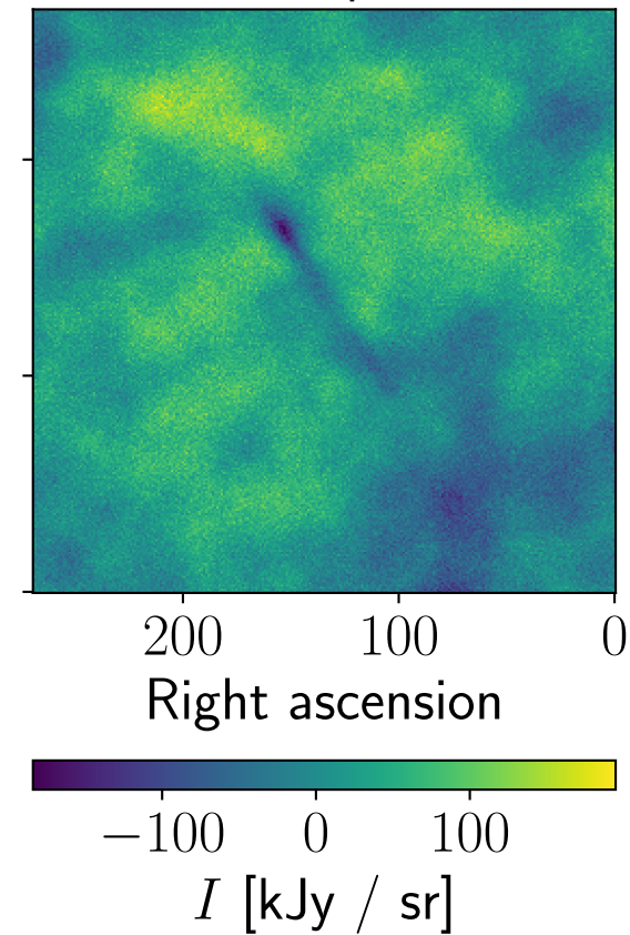
Residual, ACT, pa5, 150 GHz
