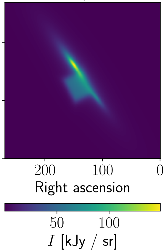
Model, ACT, pa5, 150 GHz
