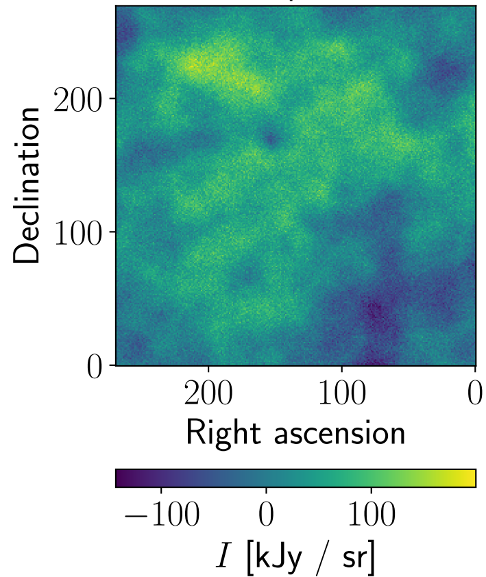
Data, ACT, pa5, 150 GHz
