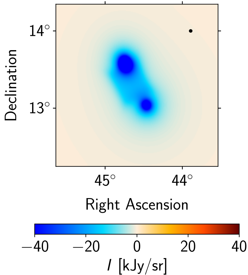
Model: ACT 150 GHz
