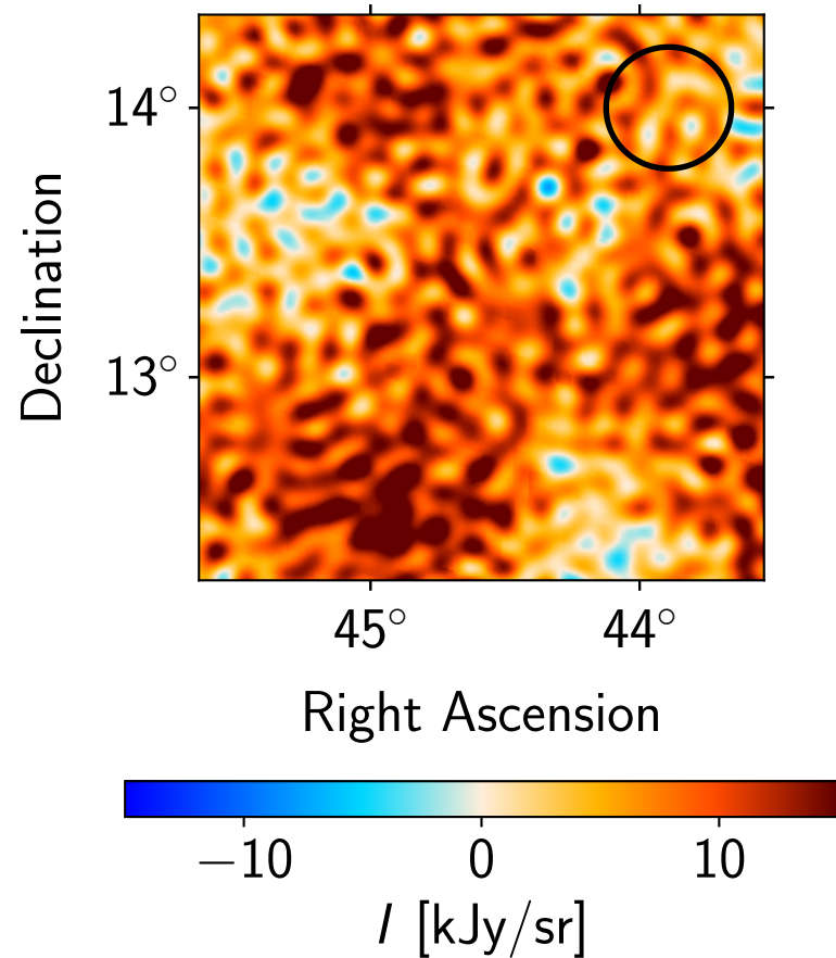
Residual: Planck 44 GHz
