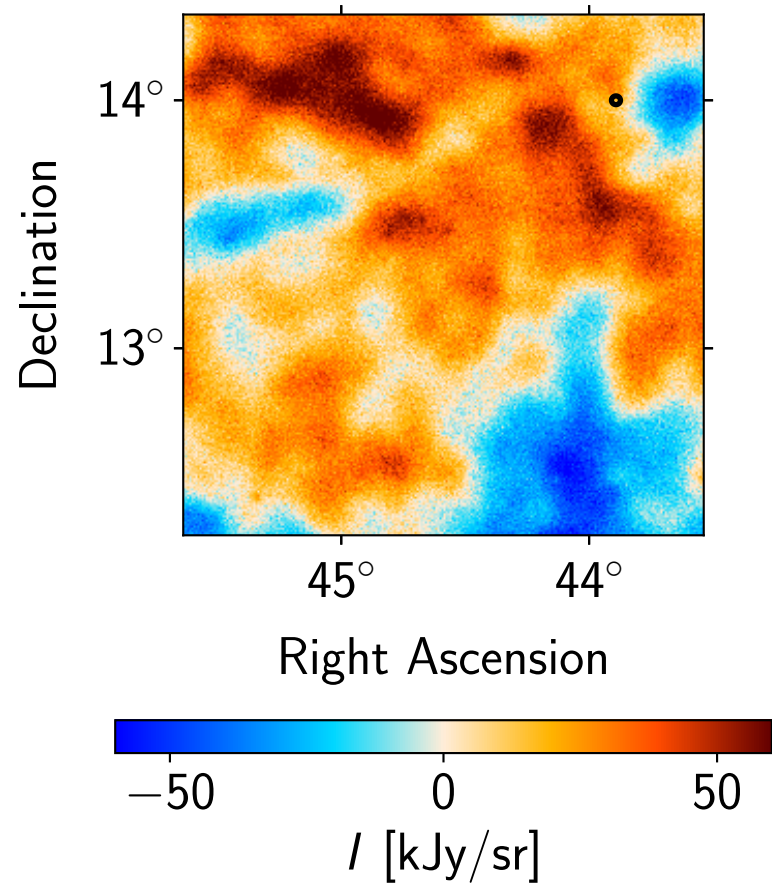
Residual: ACT 90 GHz
