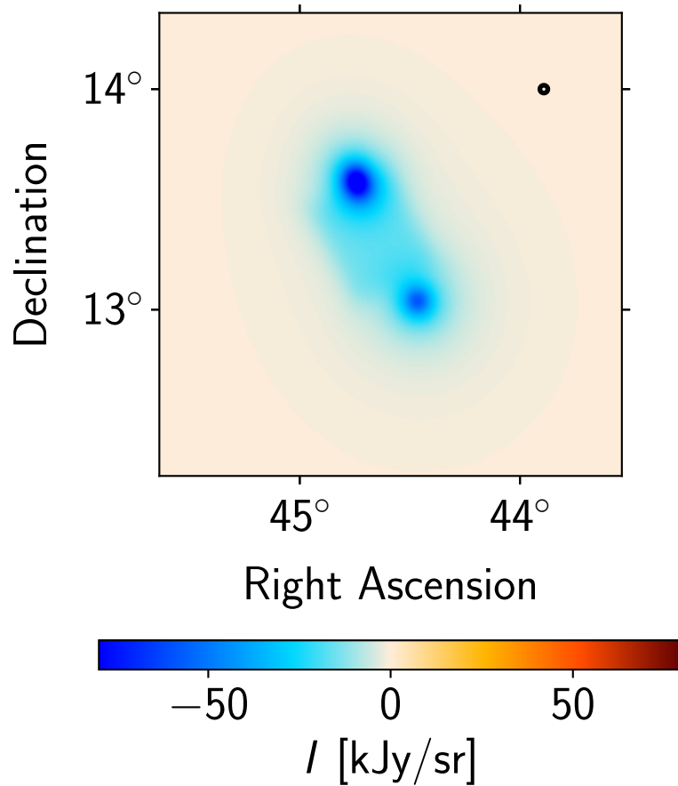
Model: ACT 90 GHz
