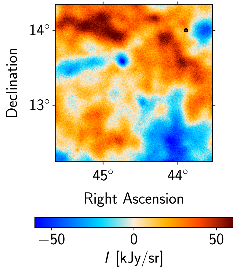
Data: ACT 90 GHz
