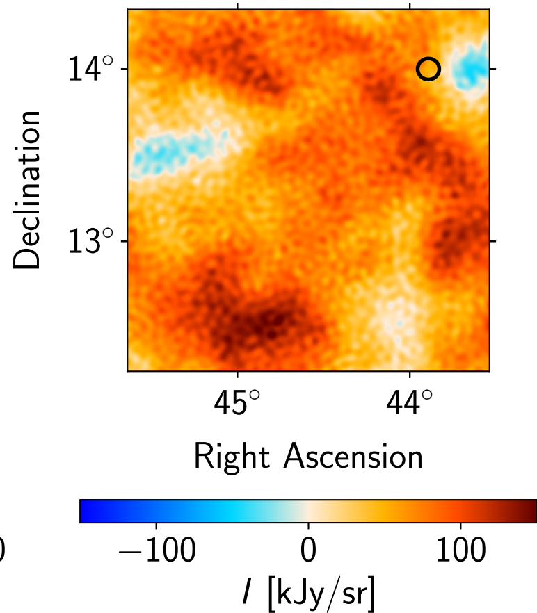
Residual: Planck 143 GHz
