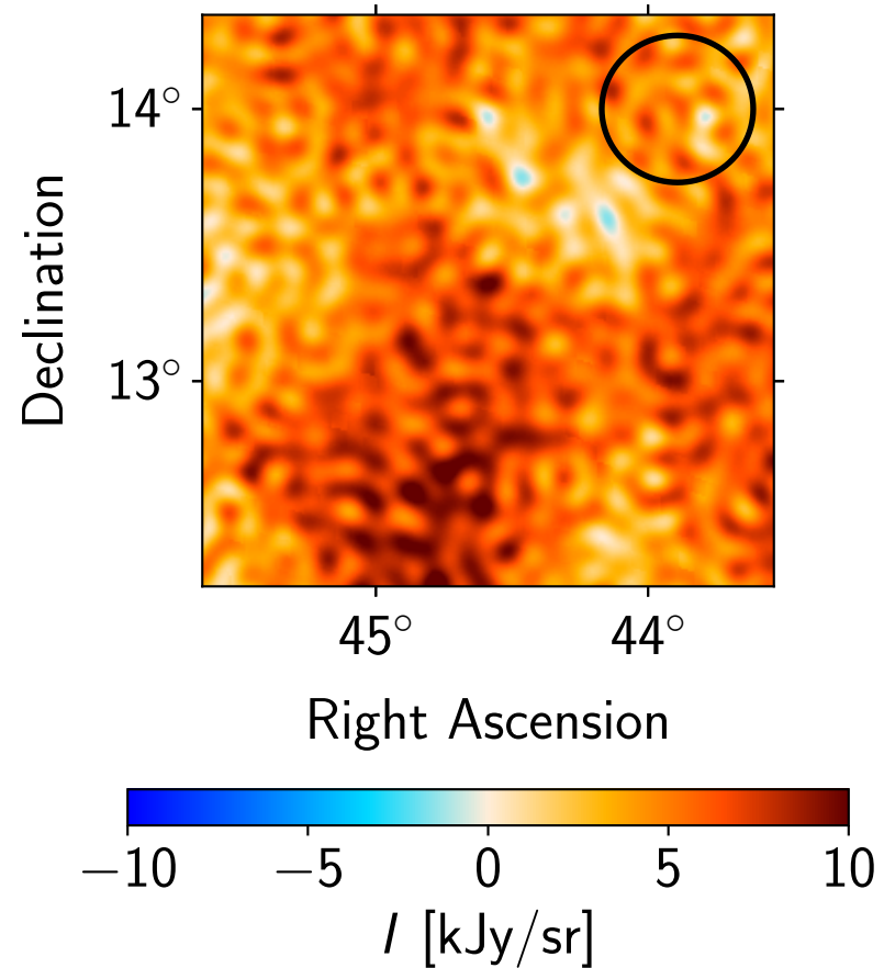
Residual: Planck 30 GHz
