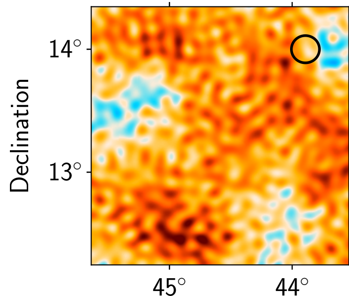
Residual: Planck 70 GHz
