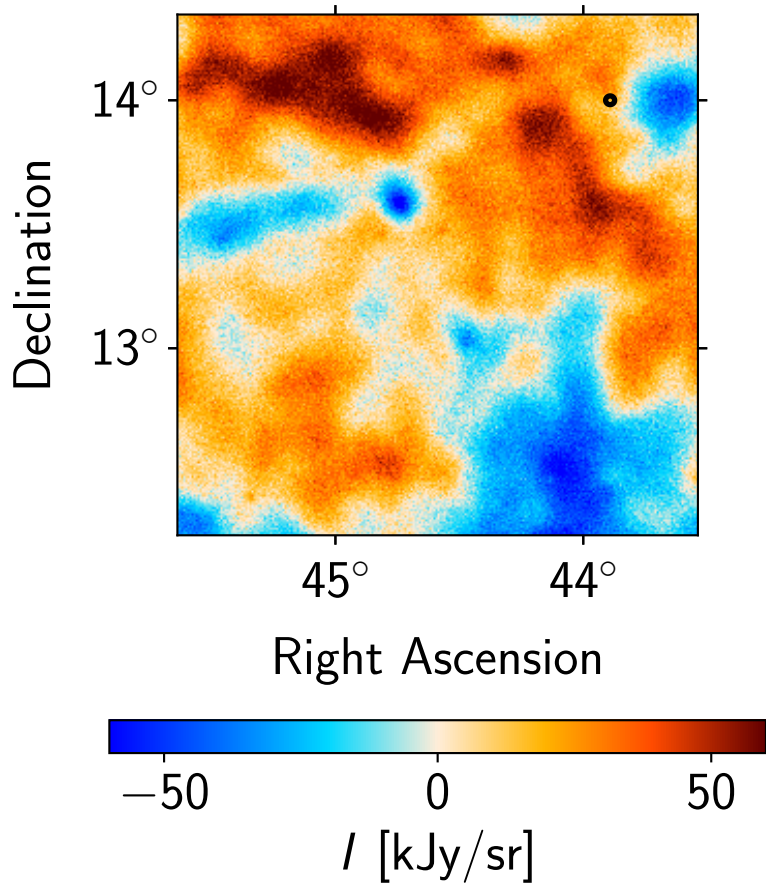
Data: ACT 90 GHz
